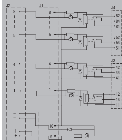
RSM-8 12 V+/24 V+/48 V+ 1C0 RSM-8I 24 V+ RSM-8 24 V+ BASE
