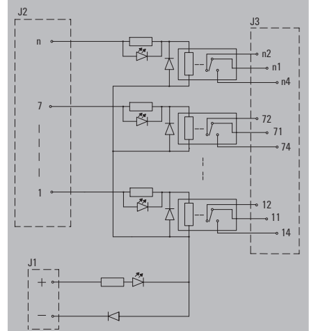
RSMS-8 12 V+/24 V+/48 V+ 1CO RSMS-16 12 V+/24 V+/48 V+ 1CO RSMS-8 24 V+ BASE RSMS-16 24 V+ BASE
