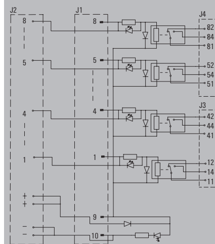
RSM-8 12 V-/24 V-/48 V- 1C0
