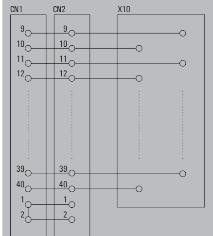
Schematic for 1371470000/1371500000
